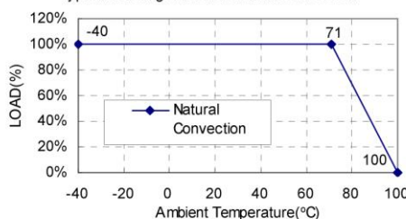
Typical Derating curve for Natural Convection
