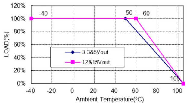
Fig2. Typical Derating Curve for Naturel Convection
