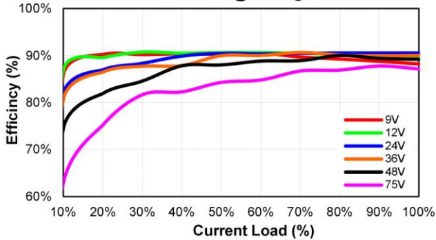
CQB50W8-36S12 Eff Vs Io @25 Deg. C
