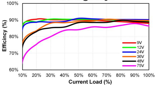
CQB50W8-36S15 Eff Vs Io @25 Deg. C
