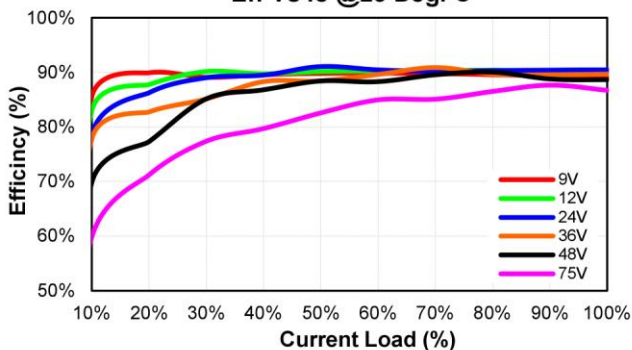
CQB50W8-36S28 Eff Vs Io @25 Deg. C
