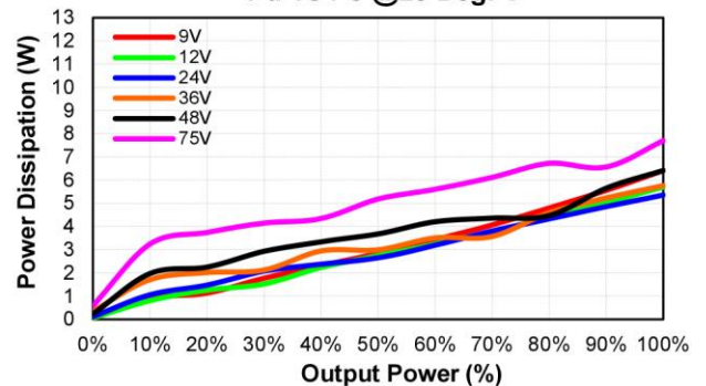
CQB50W8-36S24 Pd Vs Po @25 Deg. C
