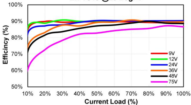
CQB50W8-36S24 Eff Vs Io @25 Deg. C
