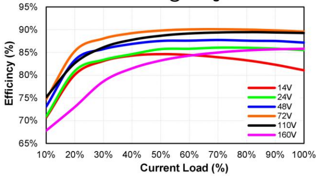
CHB200W12-72S12 Eff Vs Io @25 Deg. C
