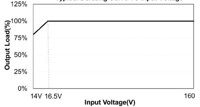
Typical Derating Curve VS Input Voltage
