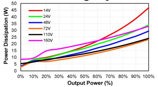
CHB200W12-72S12 Pd Vs Po @25 Deg. C
