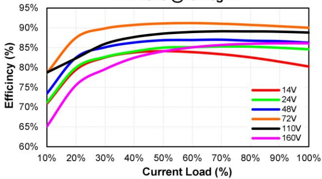
CHB200W12-72S15 Eff Vs Io @25 Deg. C
