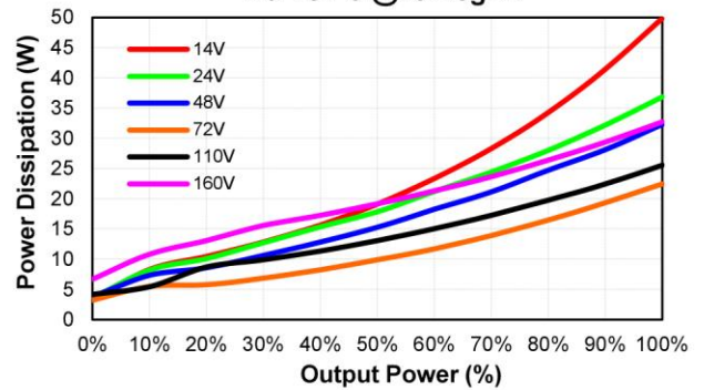
CHB200W12-72S15 Pd Vs Po @25 Deg. C
