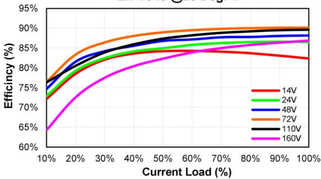
CHB150W12-72S48 Eff Vs Io @25 Deg. C
