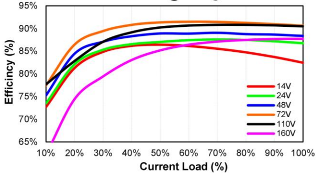
CHB150W12-72S12 Eff Vs Io @25 Deg. C
