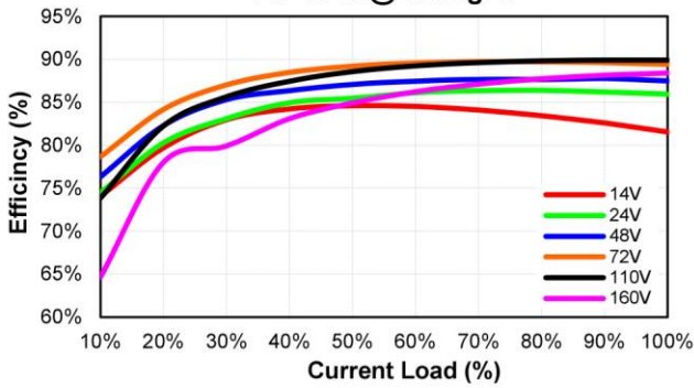
CHB150W12-72S24 Eff Vs Io @25 Deg. C
