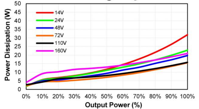
CHB150W12-72S12 Pd Vs Po @25 Deg. C
