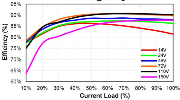
CHB150W12-72S15 Eff Vs Io @25 Deg. C
