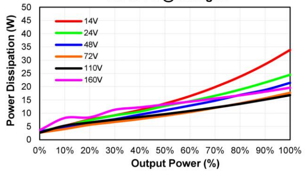
CHB150W12-72S24 Pd Vs Po @25 Deg. C
