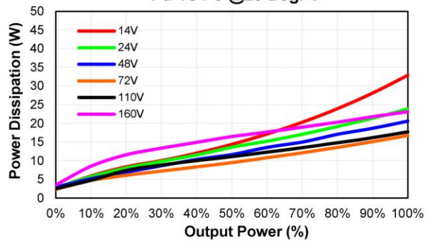
CHB150W12-72S48 Pd Vs Po @25 Deg. C
