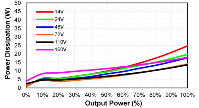
CHB150W12-72S05 Pd Vs Po @25 Deg. C
