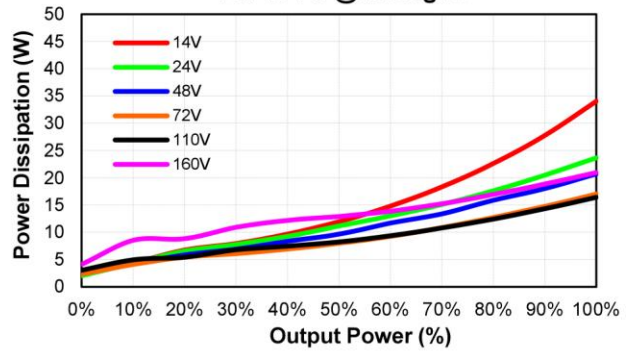
CHB150W12-72S15 Pd Vs Po @25 Deg. C
