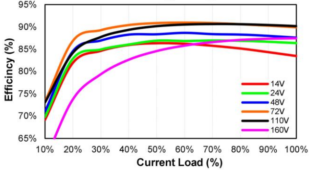
CHB150W12-72S05 Eff Vs Io @25 Deg. C
