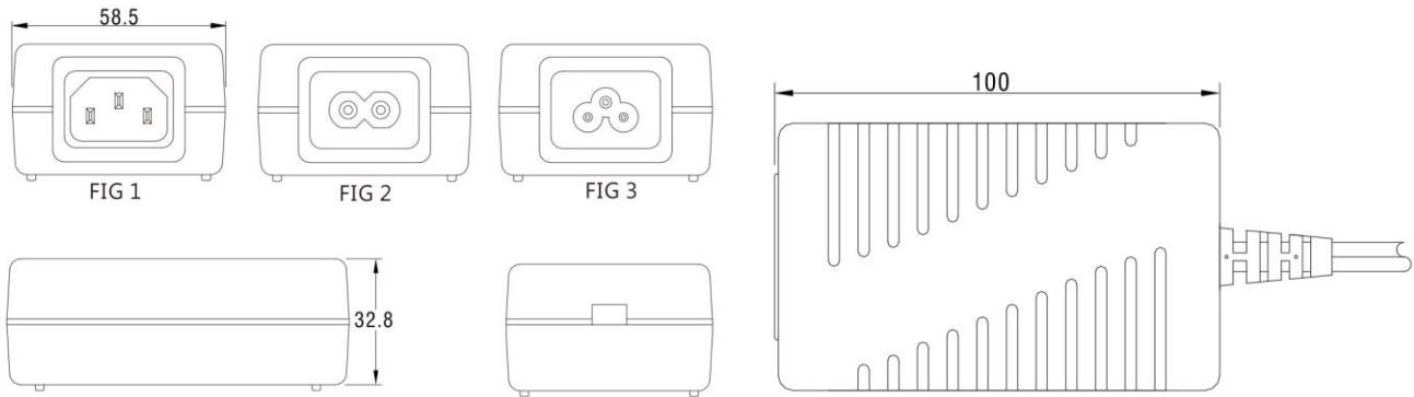
FIG 2: IEC-320-C8
