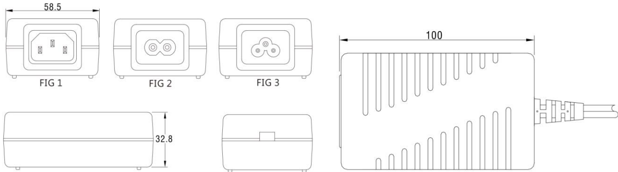
FIG 2: IEC-320-C8
