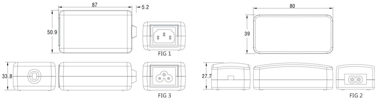
FIG 1: IEC-320-C14
