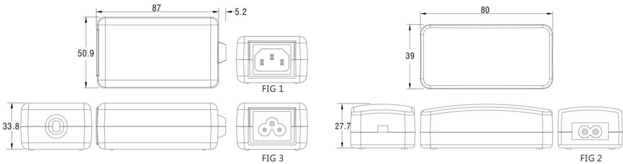
FIG 1: IEC-320-C14
