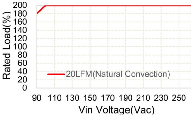
CFM81S120-CA Derating Curve for Natural Convection
