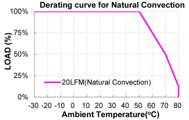
CFM81S150/240/480-CA Derating Curve for Natural Convection
