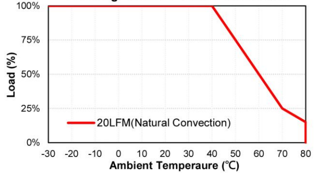
CFM81S150/240/480-CA Derating Curve for Natural Convection
