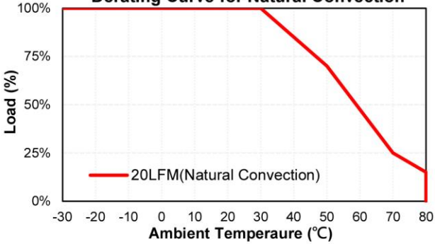
CFM81S120-CA Derating Curve for Natural Convection
