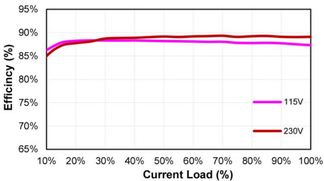
CFM81S120 (Eff Vs Io)
