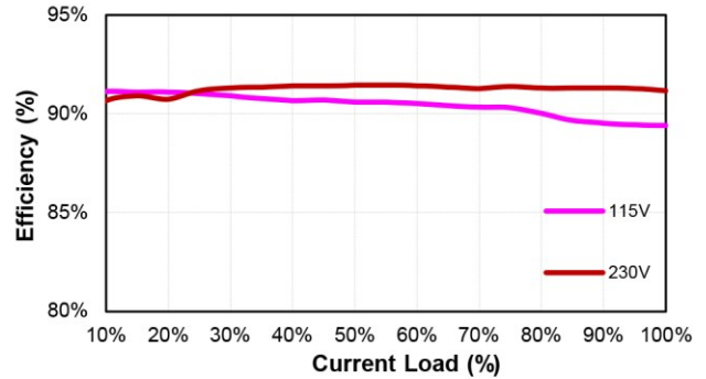
CFM70S120 (Eff Vs Io)
