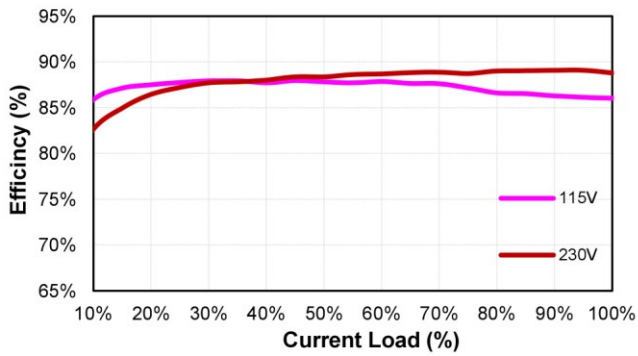
CFM20S480 (Eff Vs Io)
