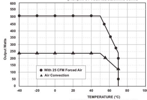
(FIG.2) TEMPERATURE DERATING CURVE
