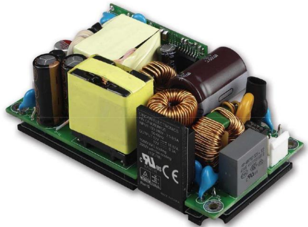
CFM200MXXX (Open Frame type)
