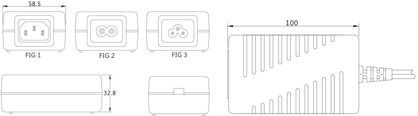
FIG 1: IEC-320-C14
