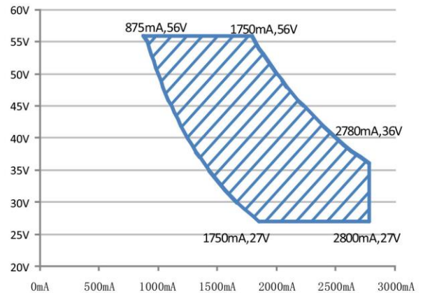
◎ XLG-100-H
