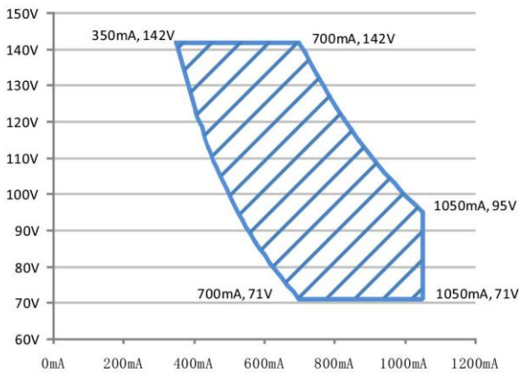
◎ XLG-100-L
