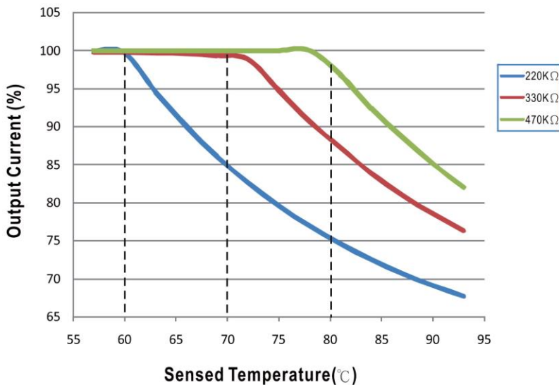
NTC derating curve
